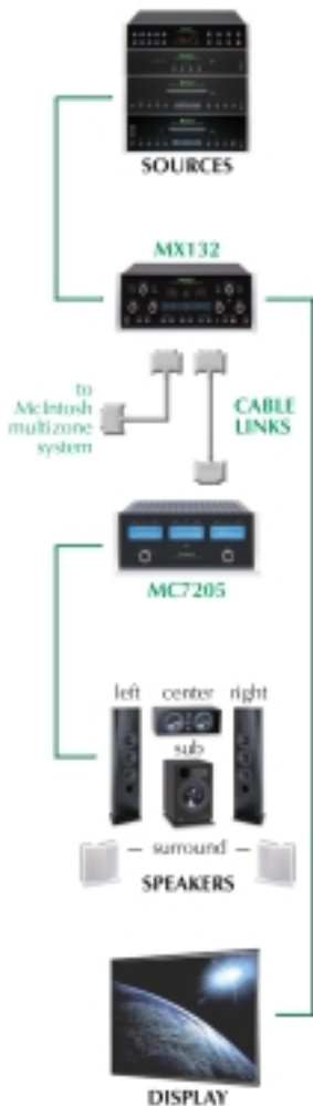
All it takes is one cable to join the MX132 and the MC7205... and one more to link a home theater to a multizone system.
